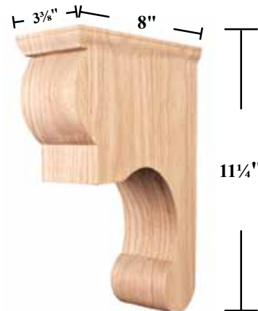
COR-SG11 Specie: A, C, M, R 3 3/8"w x 11 1/4"h x 8"d
